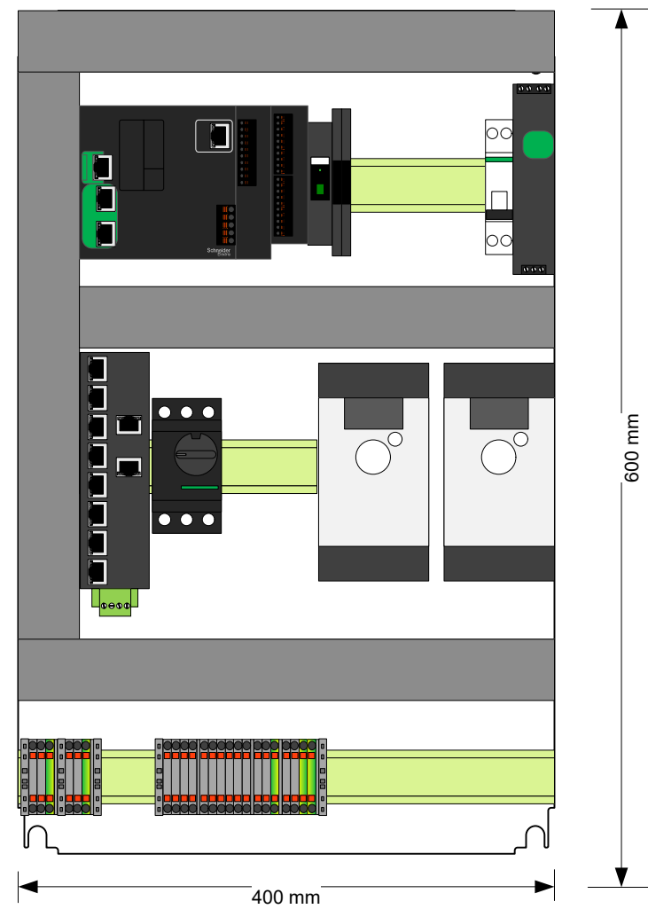
PLATE LAYOUT
