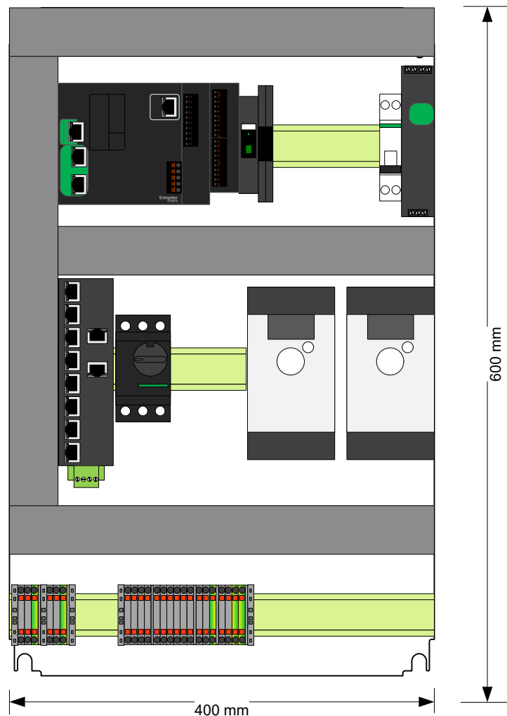
PLATE LAYOUT
